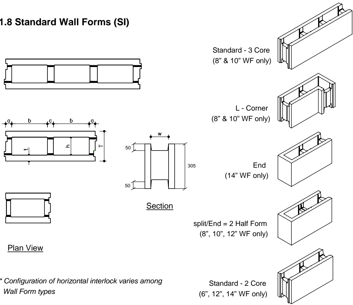
Figure 1.3 – Standard Wall Form Schematic (SI)
